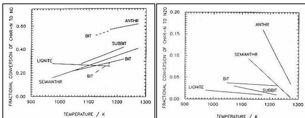
Figure 4.46 Conversion of char-N to NO ( left ) and N 2 O ( right ) versus temperature for FBC, fuels ranging from lignite to anthracite. (pictures from Johnsson, 1994)
