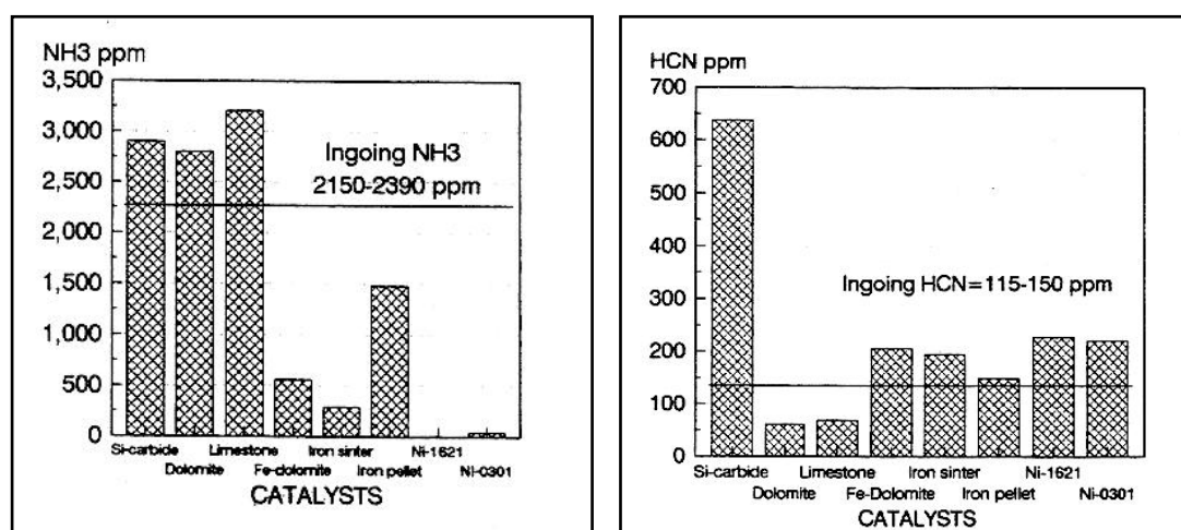
Figure 4.52 Effectivity of catalysts for in situ \text{NH}_3 and \text{HCN} conversion in fluidised bed gasification (of peat and biomass) (pictures from Leppälahti et al. , 1991)
