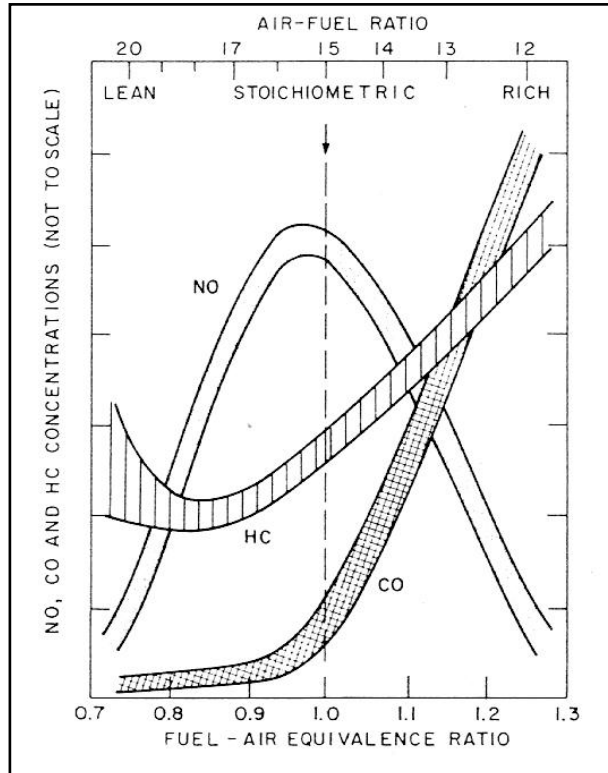
Figure 4.62 Effect of fuel / air equivalence ( \lambda = 1/\text{air factor} ) on NO, CO and hydrocarbon emissions from a spark-ignition engine (picture from Heywood, 1988)
