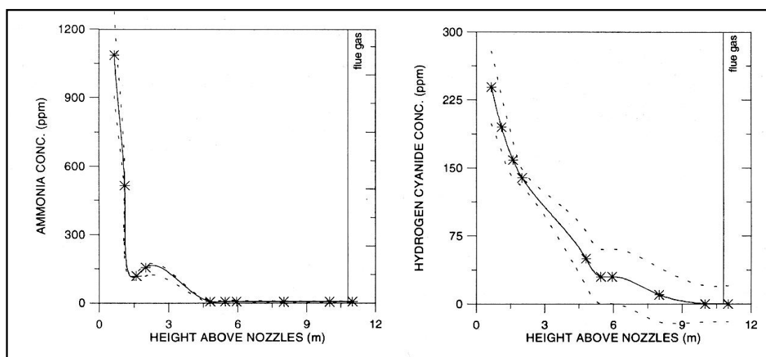
Figure 4.41 Typical measurement data for \text{NH}_3 and \text{HCN} concentration profiles in a 12 MW CFBC boiler firing bituminous coal. Bed temperature 850^\circ\text{C} , air factor 1.2-1.25, primary air factor 0.7-0.75 (picture from Åmand and Leckner 1994)
