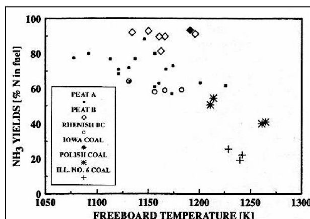
Figure 4.50 \text{NH}_3 conversion of fuel nitrogen from pressurized gasification in air. Pressure 4 ~ 9 bar (picture from Leppälähti and Koljonen, 1991)
