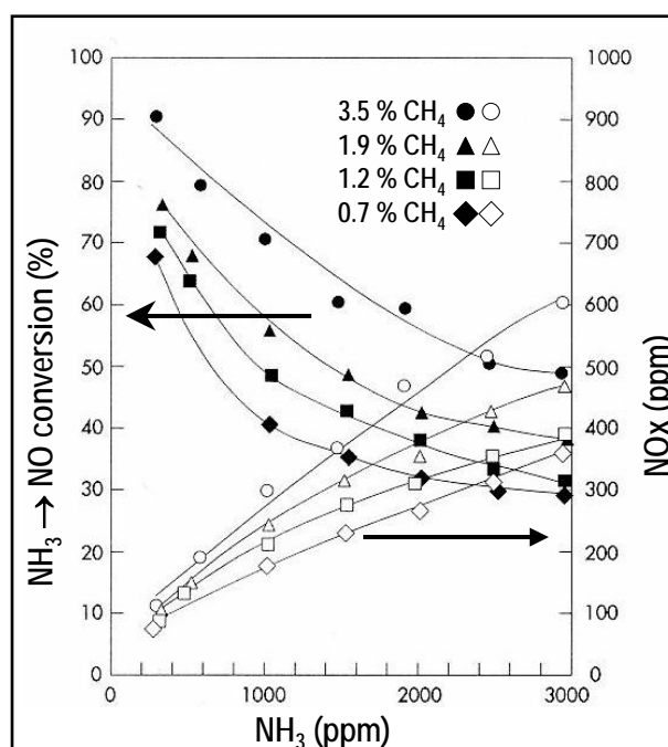
Figure 4.51 Effects of concentrations of ammonia and methane on ammonia \text{NO} conversion and \text{NO} emission at combustion of gasification gas. Data given holds at atmospheric pressure for the low \text{NO}_x burner of a gas turbine under development. Total air factor 2.0. (picture from Nakata et al. , 1994)
